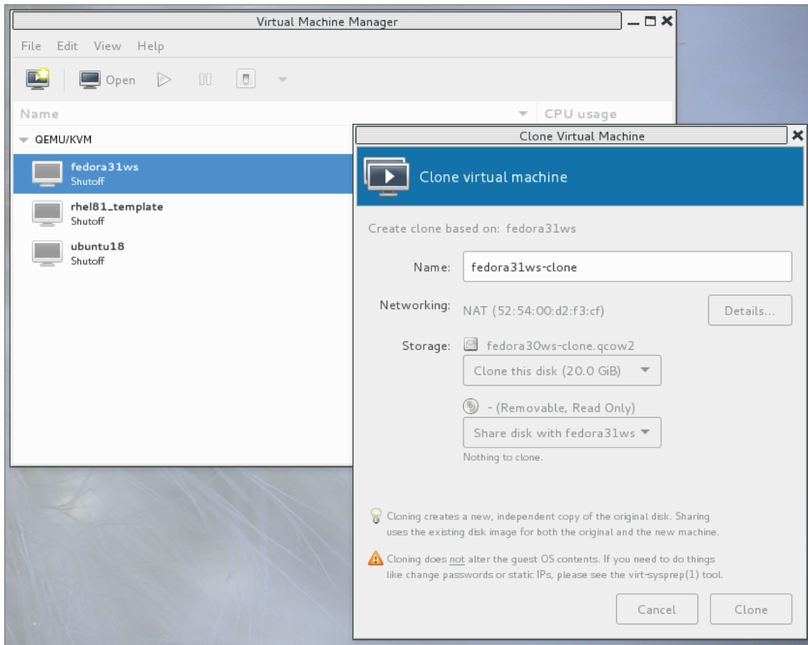
FIGURE 28.1 Cloning lets you save a permanent copy of a cloud instance.
