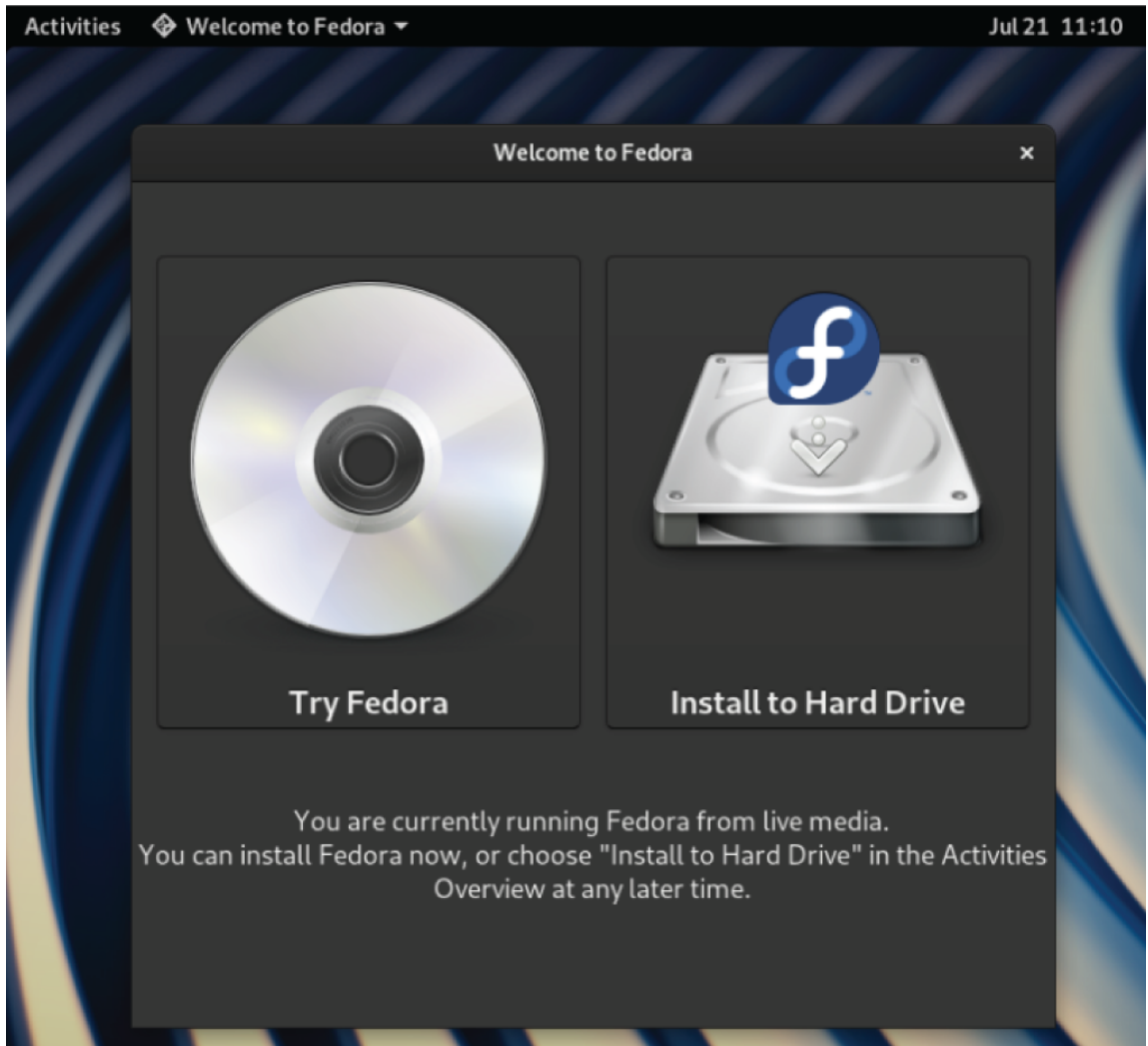
FIGURE 9.1 Start the installation process from Live media.
