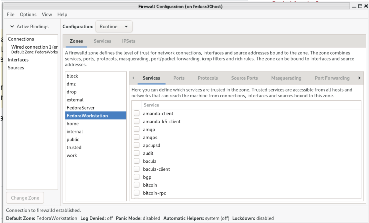
FIGURE 25.1 Firewall Configuration window
